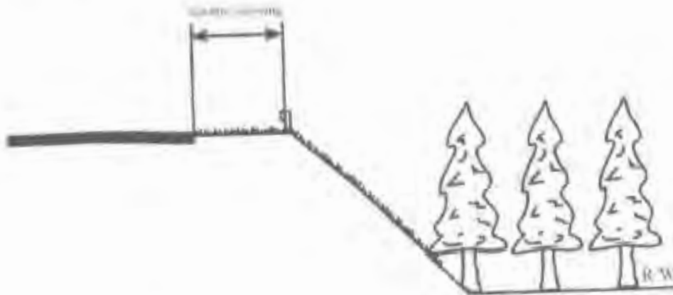
TYPICAL FILL SECTION WITH GUARDRAIL NEAR SHOULDER POINT For Swath and Ditch Contracts:
